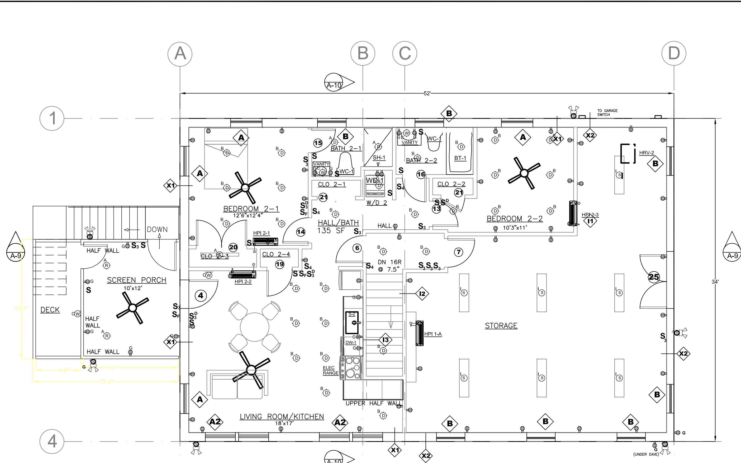
UPPER LEVEL PLAN SCALE: \frac{3}{16}'' = 1'0''
